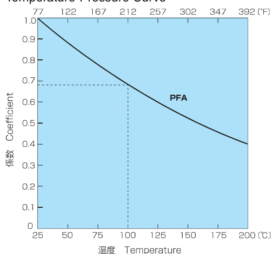
Temperature-Pressure Curve
